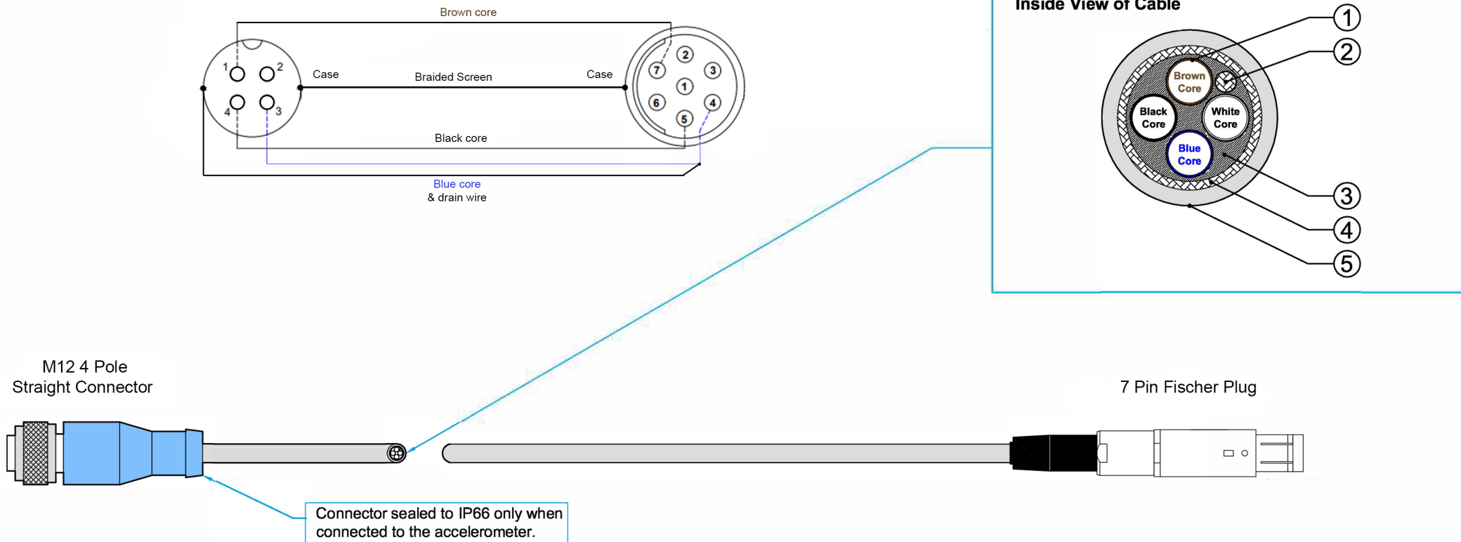
Materials of Cable: C01-001 PUR cable
