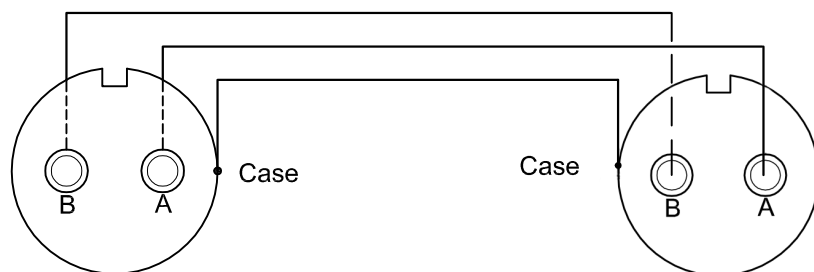
Outside View of Connector
