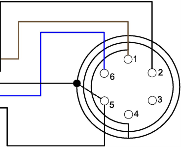
Front view of 6 Pin Fischer Connector
