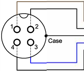
Front view of 4 Pin M12 Connector
