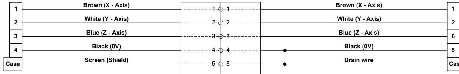
Female 4 Pin M12 (HS-173)
