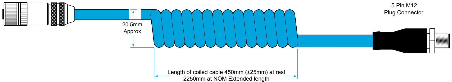
5 Core Polyurethane Screened Coiled Cable
