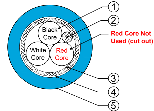
Cross Sectional View of Cable
