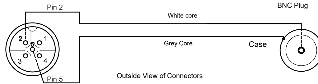
5 Pin M12 Plug Connector
