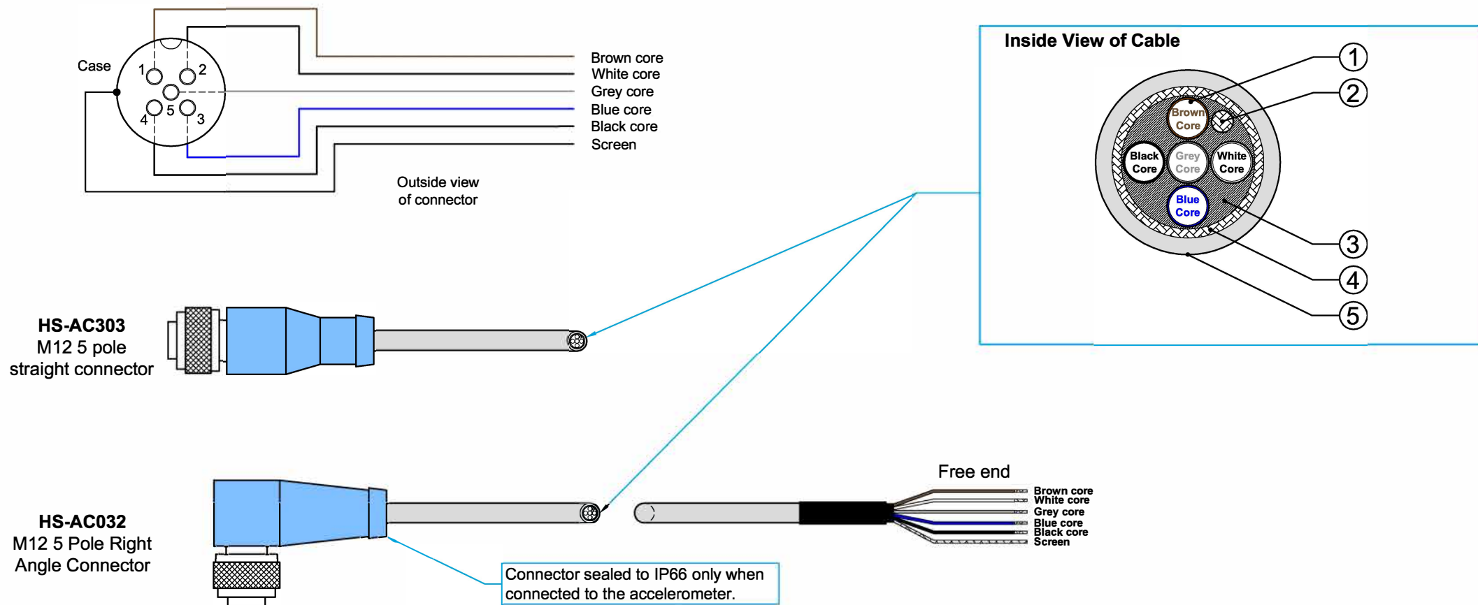
Materials of Cable: C01-030 Screened PUR Cable
