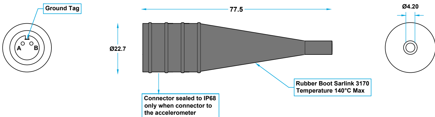
Front View
