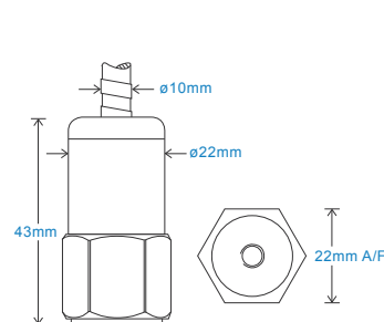
Connection Details
